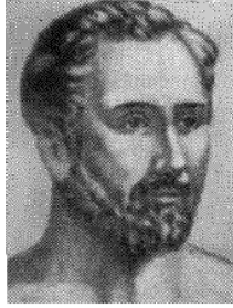
Pythagoras
